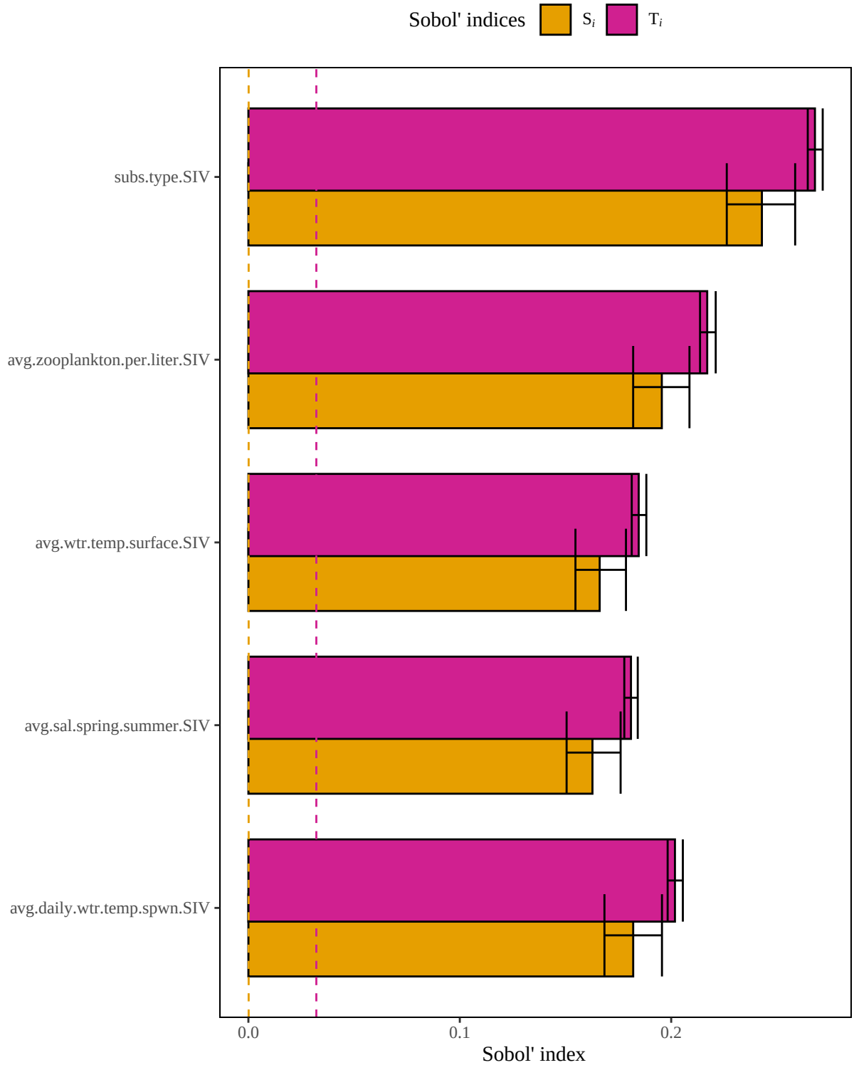
Figure 5. Results of a sensitivity analysis for the blueherringJuvAndSAEL model based on a geometric mean structure. Dashed lines represent baseline numerical approximation error for S_i and T_i ( i.e. , dummy variables).
