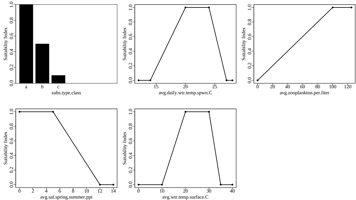
Figure 1. Suitability index graphs for variables included in the blueherringJuvAndSAEL model in ecorest .
